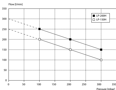
Flow Curves
